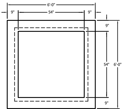
ROOF PLAN TYPE 2 - MC-102 (75-500 KVA TRANSFORMER COVER) PICK WEIGHT - 1,200#
