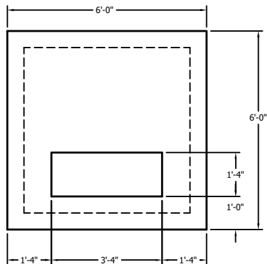
ROOF PLAN MC-101 (75-500 KVA TRANSFORMER COVER) PICK WEIGHT - 2,700#
