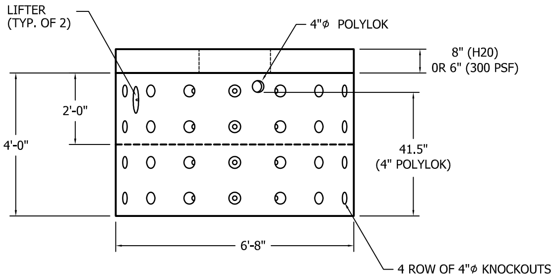
FRONT VIEW (4 FT. HIGH)
