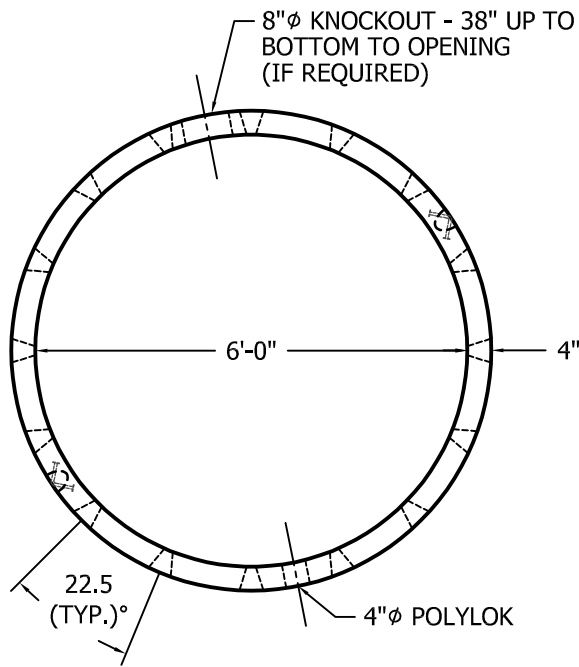
PLAN VIEW (DRY WELL RING)
