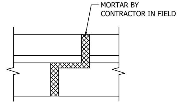
JOINT DETAIL 1" = 1'-0"
