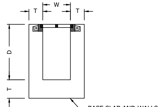
SECTION B-B 1" = 1'-0"
