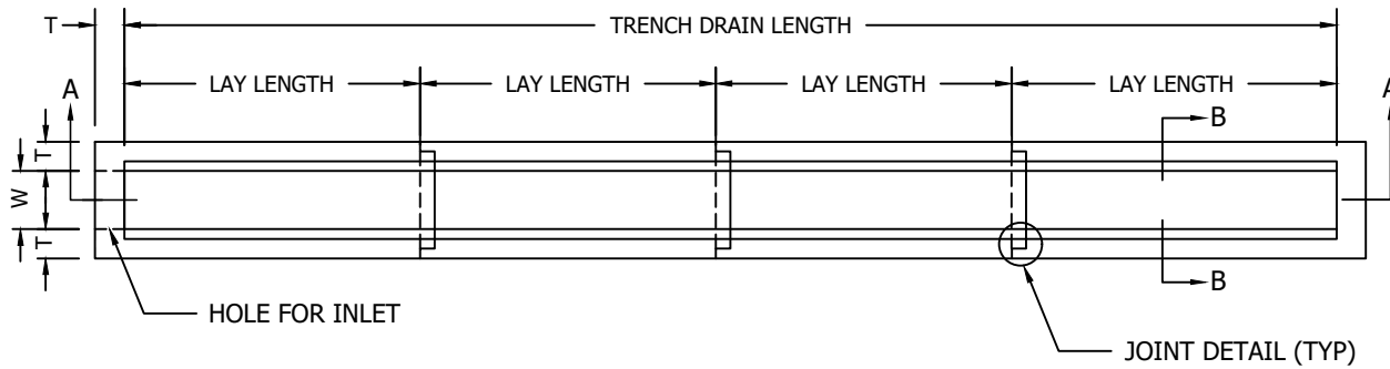
PLAN 1" = 1'-0"
