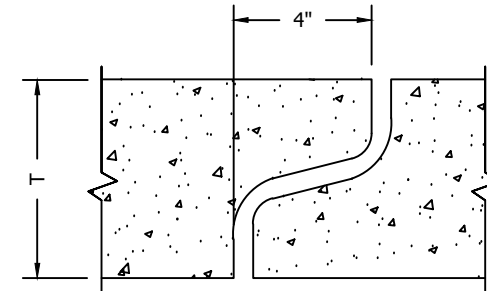
JOINT DETAIL NTS
