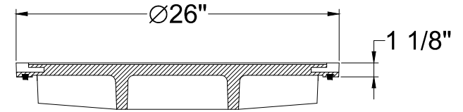
COVER SECTION A-A
