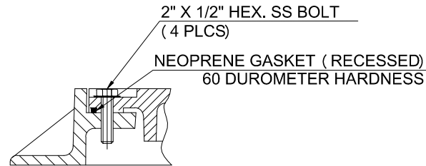
DETAILS OF "X"
