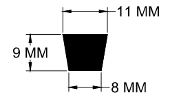
DETAILS OF GASKET
